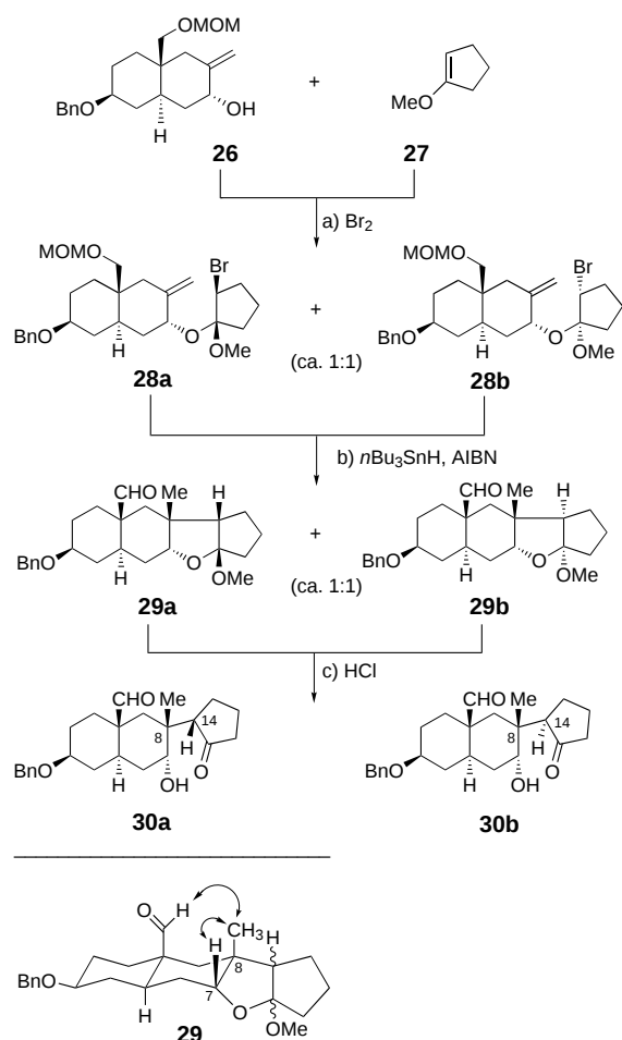
Scheme 4. Synthesis of model systems 30a and 30b . a) 27 (10.0 equiv), \text{Br}_2 (5.0 equiv), N,N -dimethylaniline (6.0 equiv), \text{CH}_2\text{Cl}_2 , 25^\circ\text{C} , 12 h, 79% (mixture of diastereoisomers, ca. 1:1); b) n\text{Bu}_3\text{SnH} (1.6 equiv), AIBN (0.14 equiv), 0.004M in toluene, 12 h, 100^\circ\text{C} , 79%; c) 1M aq. \text{HCl}/\text{THF} (1:3.3), 25^\circ\text{C} , 144 h, 70% (separated diastereoisomers, 1:1).
