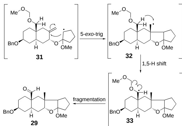
Scheme 5. Postulated mechanism for the radical-based cascade sequence 28 \rightarrow 29 .
