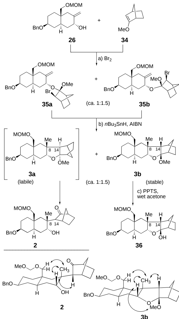
Scheme 6. Synthesis of azadirachtin model systems 2 , 3b and 36 . a) 34 (5.0 equiv), \text{Br}_2 (4.3 equiv), N,N -dimethylaniline (4.65 equiv), \text{CH}_2\text{Cl}_2 , 25^\circ\text{C} , 2 h, 71% (mixture of diastereoisomers, ca. 1.5:1); b) n\text{Bu}_3\text{SnH} (1.3 equiv), AIBN (0.2 equiv), 0.003M in toluene, 15 min, 110^\circ\text{C} , 70% (mixture of diastereoisomers, ca. 1.5:1); c) PPTS (0.05 equiv), acetone/ \text{H}_2\text{O} (10:1), 65^\circ\text{C} , 72 h, 85%.
