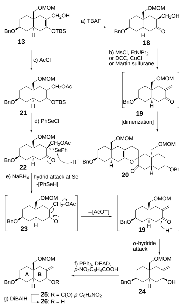
Scheme 3. Synthesis of allylic alcohol 26 . a) TBAF (1.1 equiv), THF/AcOH (100:1), 25^\circ\text{C} , 6 h, 100%; b) e.g., \text{MsCl} (2.5 equiv), \text{Et}_3\text{N}/\text{Pr}_2 (7.5 equiv), \text{CH}_2\text{Cl}_2 , 25^\circ\text{C} , 24 h, 83%; c) \text{AcCl} (3.0 equiv), py (10.0 equiv), \text{CH}_2\text{Cl}_2 , 25^\circ\text{C} , 1 h, 67%; d) \text{PhSeCl} (1.1 equiv), -78^\circ\text{C} , 1 h, then 25^\circ\text{C} , 1 h; e) \text{NaBH}_4 (6.8 equiv), \text{CH}_2\text{Cl}_2/\text{MeOH} (1:1), -78^\circ\text{C} , 1 h, then 25^\circ\text{C} , 1 h, 98% (2 steps); f) \text{PPh}_3 (3.0 equiv), \text{DEAD} (3.0 equiv), p -nitrobenzoic acid (2.5 equiv), benzene, 25^\circ\text{C} , 14 h, 78%; g) \text{DIBALH} (3.1 equiv), \text{CH}_2\text{Cl}_2 , -78^\circ\text{C} , 3 h, 79%. TBAF = tetrabutylammonium fluoride, Ms = methanesulfonyl, DEAD = diethyl azodicarboxylate.
